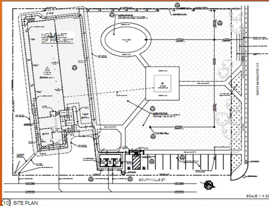
10 SITE PLAN
